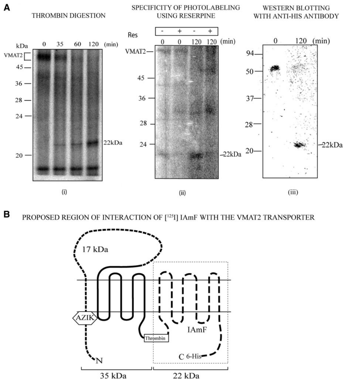
Fig. 6. Ai, time course of thrombin digestion of a [ ^{125} I]IAmF photolabeled vesicle preparation from SH-SY5Y cells transfected with hVMAT2 with an engineered thrombin site between TM6 and TM7 (Thiriou et al., 2002). ii, reserpine protection of the 22-kDa fragment, generated from thrombin digestion of photolabeled transporter. iii, Western immunoblotting of undigested and thrombin-digested photolabeled transporter with C-terminal anti-His antibody. B, the proposed sites of interaction of [ ^{125} I]IAmF with the VMAT2 molecule; also shown is the site of interaction of the inhibitor photolabel [ ^{125} I]AZIK, which derivatized Lys-20 of VMAT2 (Sievert and Ruoho, 1997).
