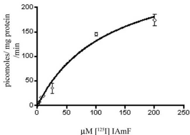
Fig. 4. Saturation uptake of [ ^{125} I]IAmF into Sf9 vesicles expressing VMAT2. The specific activity of carrier-free [ ^{125} I]IAmF was reduced by adding appropriate amounts of unlabeled IAmF to obtain high concentrations of the substrate. Vesicles were incubated with increasing concentrations of [ ^{125} I]IAmF in the presence of ATP-Mg for 15 min at 32°C and filtered using vacuum filtration on to GF-B disks. Radioactivity retained on the filter was counted in a \gamma -counter. Uptake was calculated as picomoles per milligram of protein per minute after correction of specific activity.
