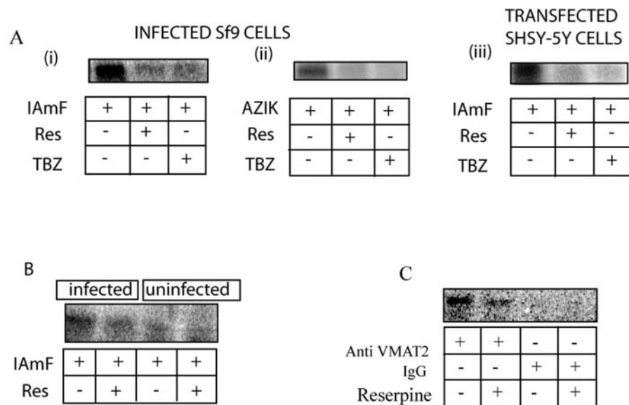
Fig. 4. Saturation uptake of [ ^{125} I]IAmF into Sf9 vesicles expressing VMAT2. The specific activity of carrier-free [ ^{125} I]IAmF was reduced by adding appropriate amounts of unlabeled IAmF to obtain high concentrations of the substrate. Vesicles were incubated with increasing concentrations of [ ^{125} I]IAmF in the presence of ATP-Mg for 15 min at 32°C and filtered using vacuum filtration on to GF-B disks. Radioactivity retained on the filter was counted in a \gamma -counter. Uptake was calculated as picomoles per milligram of protein per minute after correction of specific activity.
