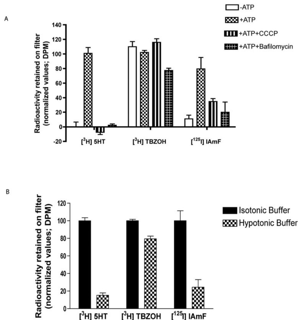
Fig. 3. A, radioactive 5-HT, TBZOH, and IAmF were allowed to interact with vesicles from infected Sf9 cells in the absence or presence of ATP (10 mM) or in the presence of bafilomycin A1 (10 \mu M) or CCCP (1 \mu M). VMAT2-specific radioactivity retained on the filter is shown normalized to values obtained in the presence of 10 mM ATP-Mg. B, demonstration of a method to distinguish between a substrate and ligand by allowing the compounds to interact with the Sf9 vesicles expressing rVMAT2, followed by isotonic or hypotonic buffer washes. Radioactivity retained on the filters is shown as normalized DPM values to the values obtained upon isotonic washes.
